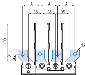
TS100, 160, 250 4P
